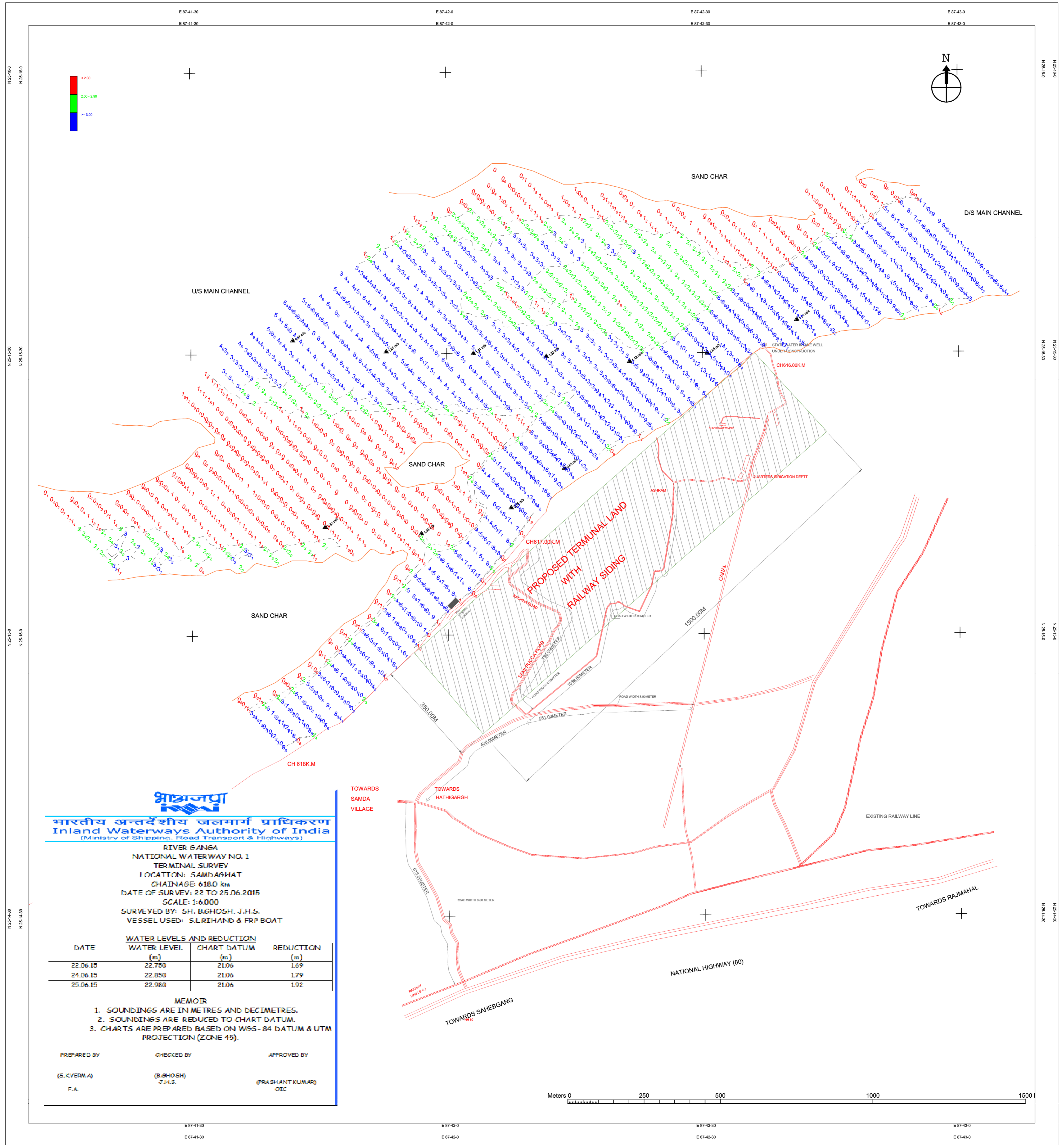
Figure 2.2: Details of Hydrographic Survey in river Ganga at Proposed Terminal at Sahibganj
